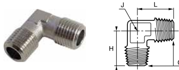
0914 / 0922 Equal Elbow Male BSPT or M5
