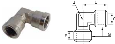
0912 Female Elbow BSPP and M5
